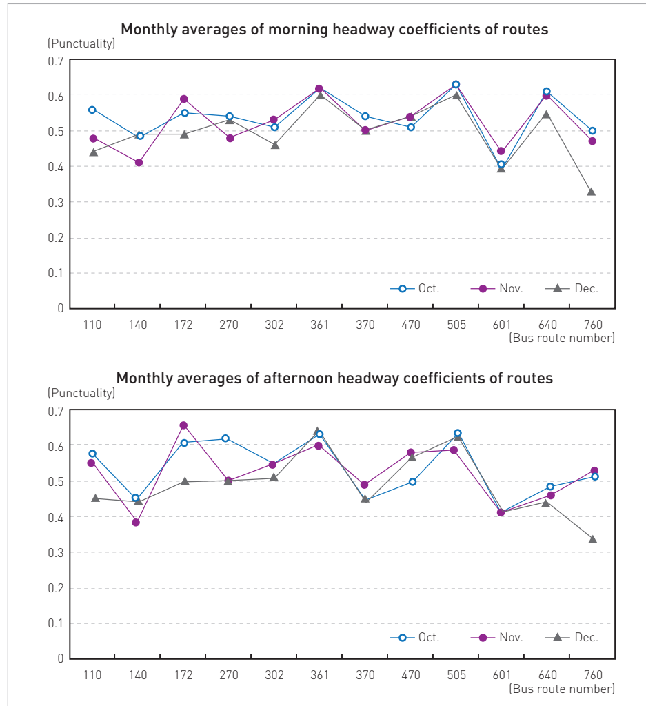
Figure 2-6. Headway coefficients
