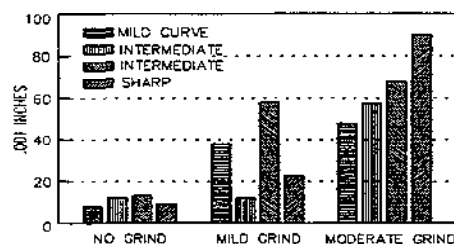
Figure 2.6.6 Preliminary High Face Gauge Wear Measurements
