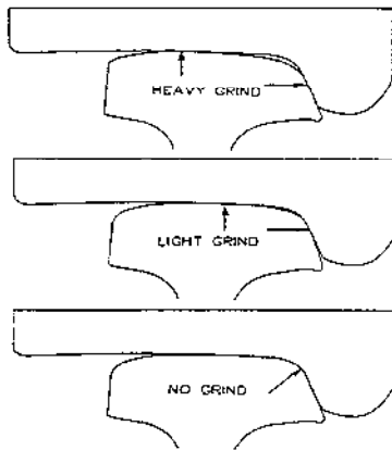
Figure 2.6.8 Three Rail Profiles Used in AAR Demonstration
