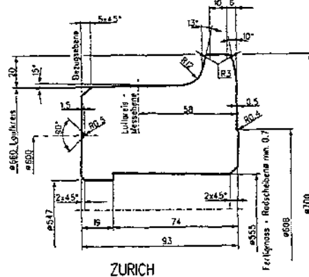
Figure 2.6.3 European Wheel Profiles
