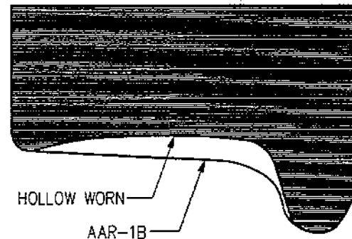
Figure 2.6.7 New AAR-1B and Hollow Worn Wheel
