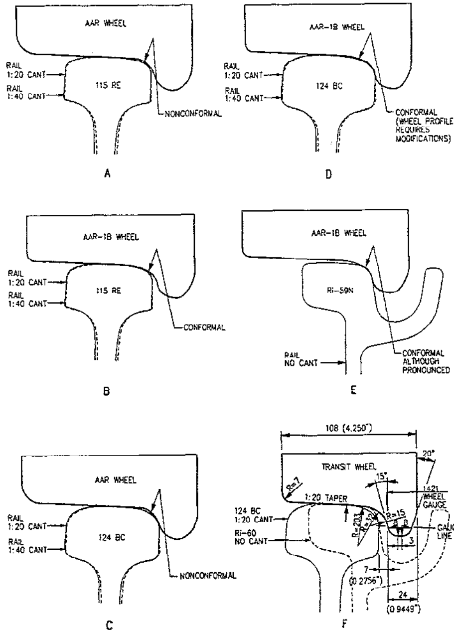
Figure 2.6.5 Wheel-Rail Interface
