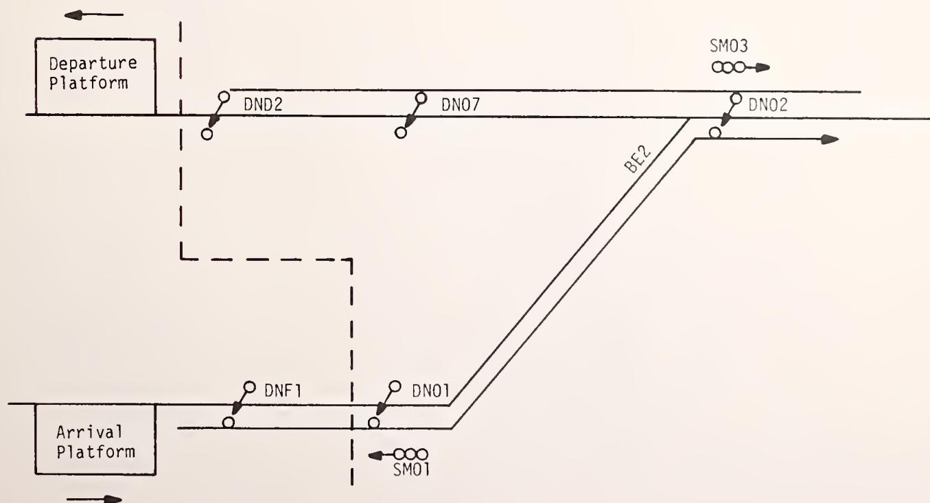
FIGURE 4-15. WEST TERMINAL
