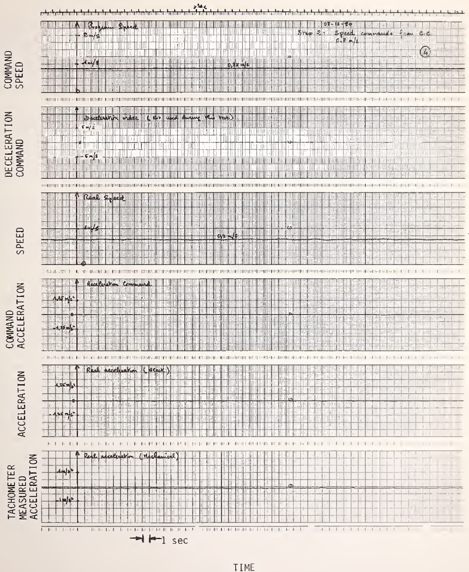
FIGURE 4-24. SPEED AND ACCELERATION PROFILES - 0.8 m/sec Comanded by CC
