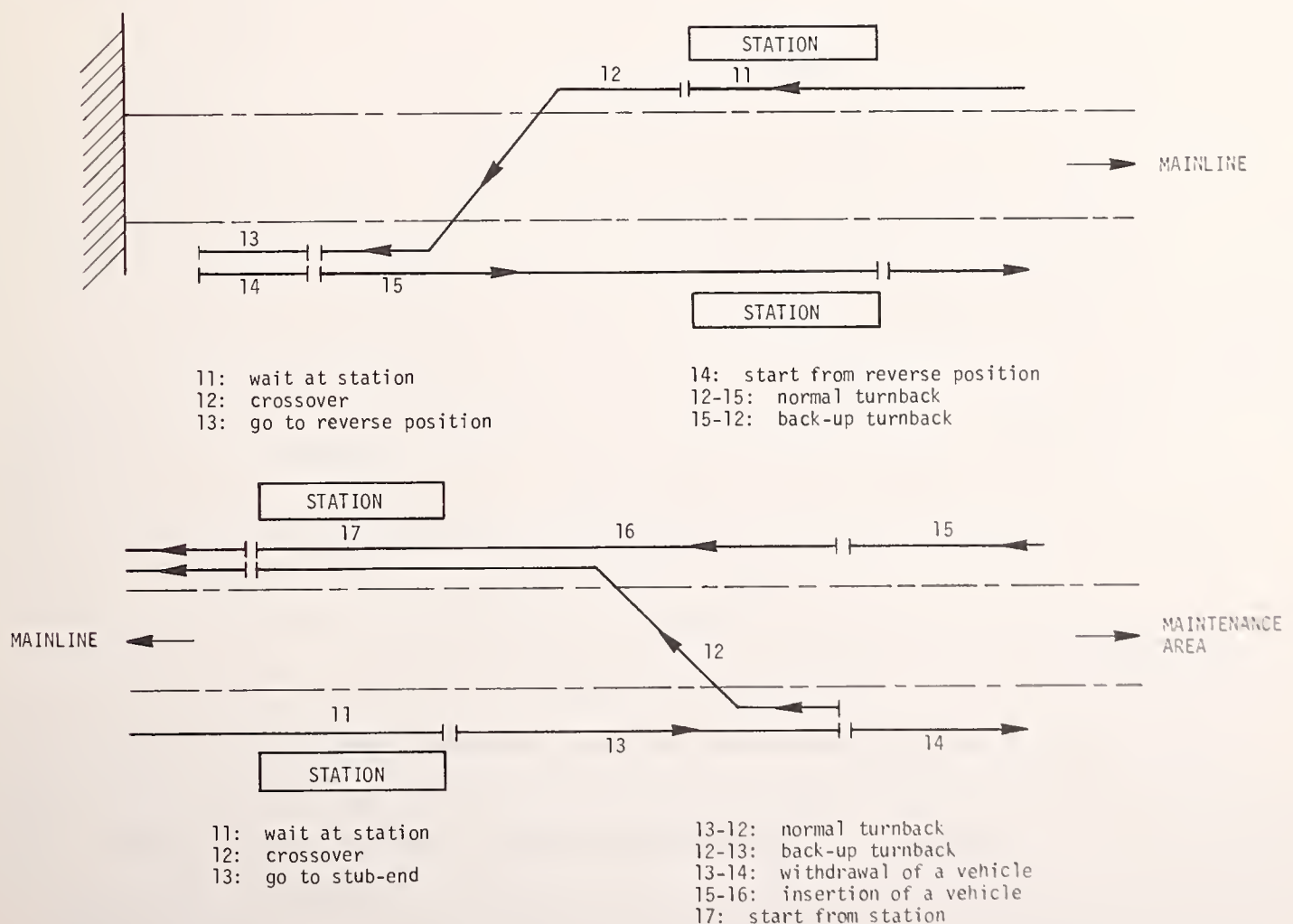
FIGURE 3-38. AUTOMATIC ROUTE OPTIONS AT TERMINALS
