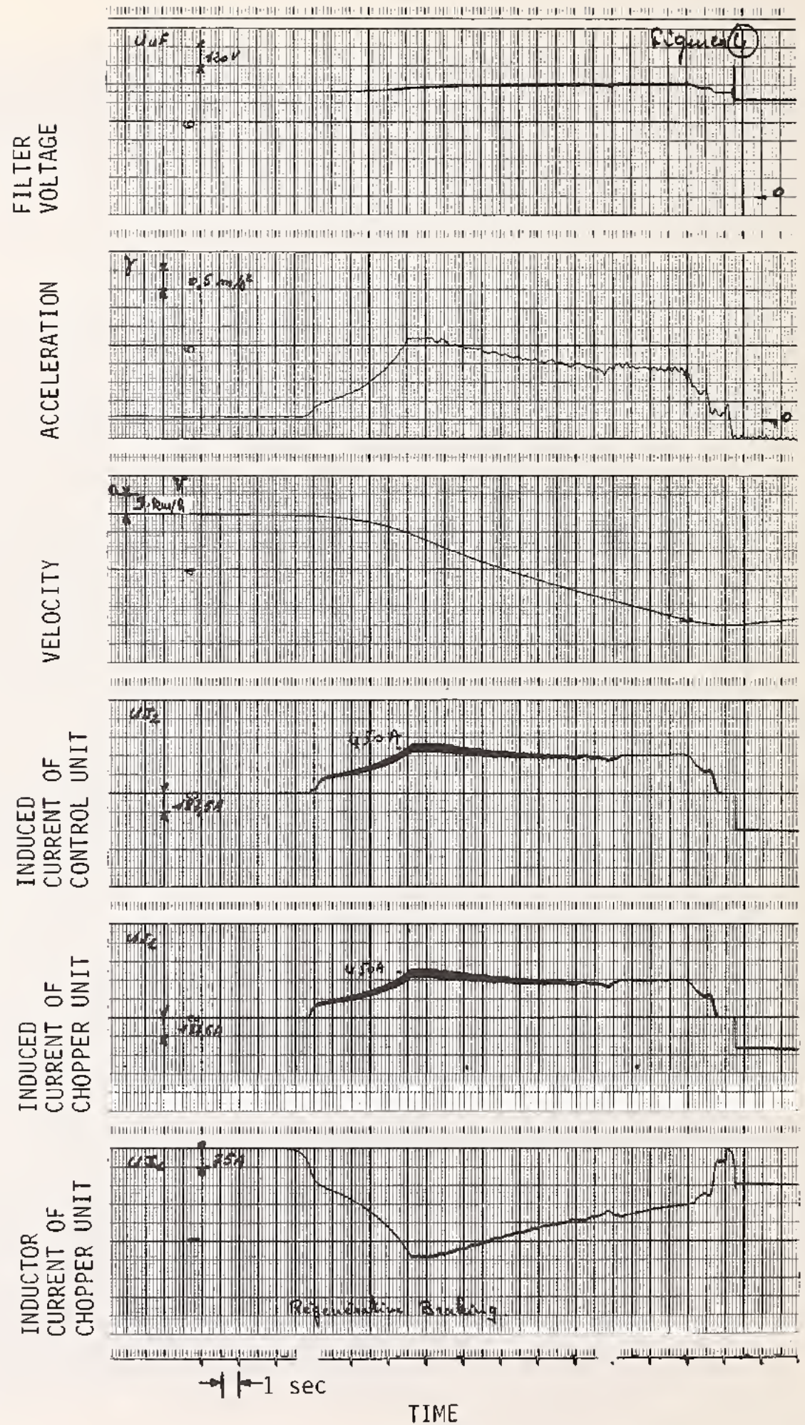
FIGURE 4-7. REGENERATIVE BRAKING-- 60 km/hr
