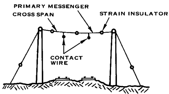
SIMPLE CROSS SPAN-SIMPLE CONTACT WIRE
