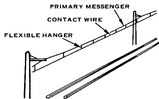
SIMPLE CATENARY SUSPENSION
