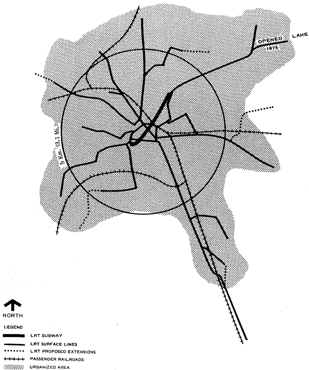
Figure 10. Hannover System
