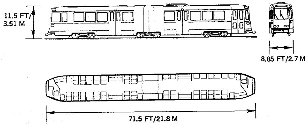
Figure 25. Boeing LRV
