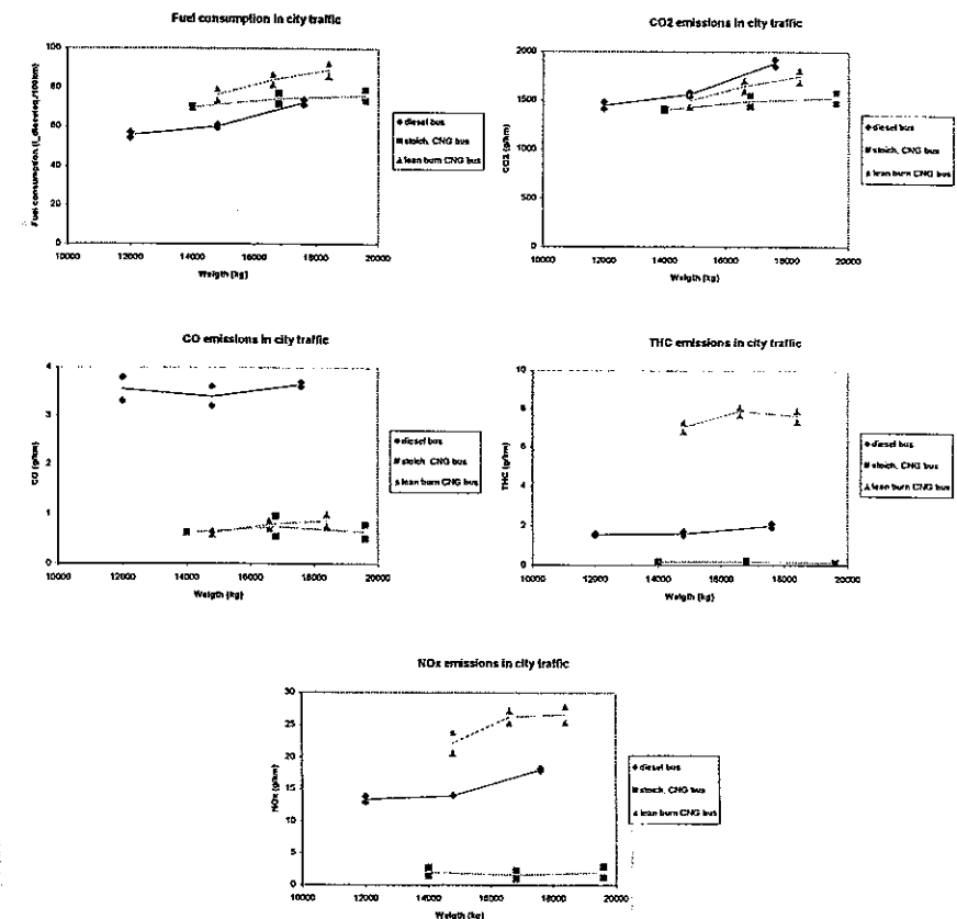
Figure 4: Effect of vehicle weight on fuel consumption and emissions
