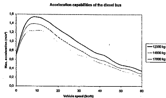
Figure 3: influence of vehicle weight on the acceleration capabilities of the diesel bus
