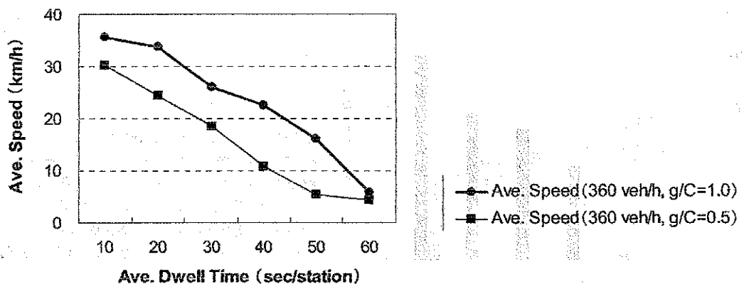
Figure 6. Case 4 : Results of Calculation for Bus Ordering System*
