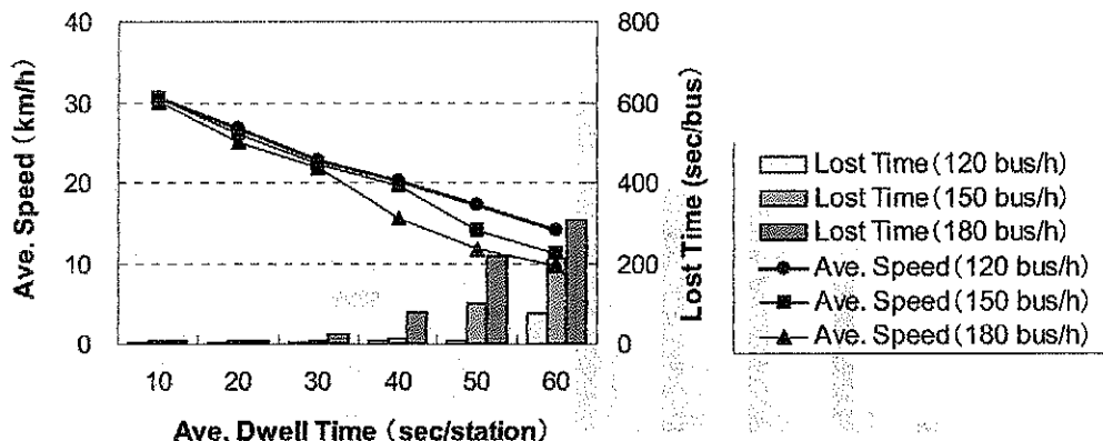
Figure 5. Case 3: Results of Calculation for Operation with Multi-Bus Bays
