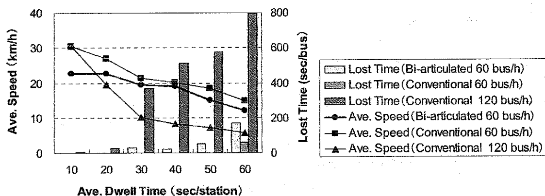
Figure 4. Case 2: Comparing Result of High Capacity Bus Operating to Case 1
