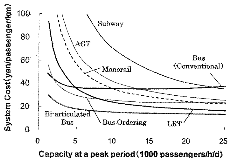
Figure 7. Relationship between Capacity at peak period and System Cost
