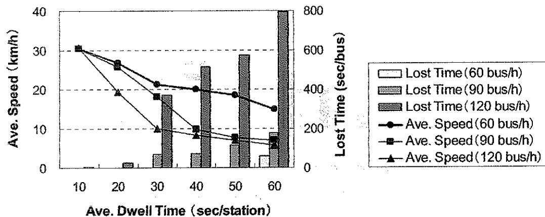
Figure 3. Case 1: Results of Calculation for Normal Service
