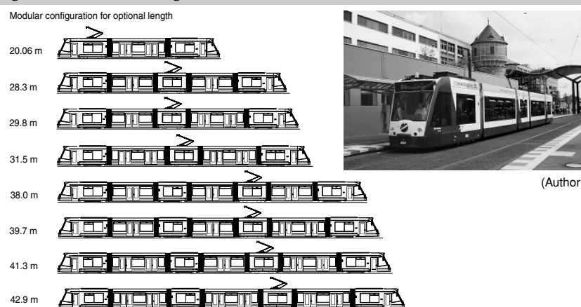
Figure 2 Modular Design of Combino Trams
