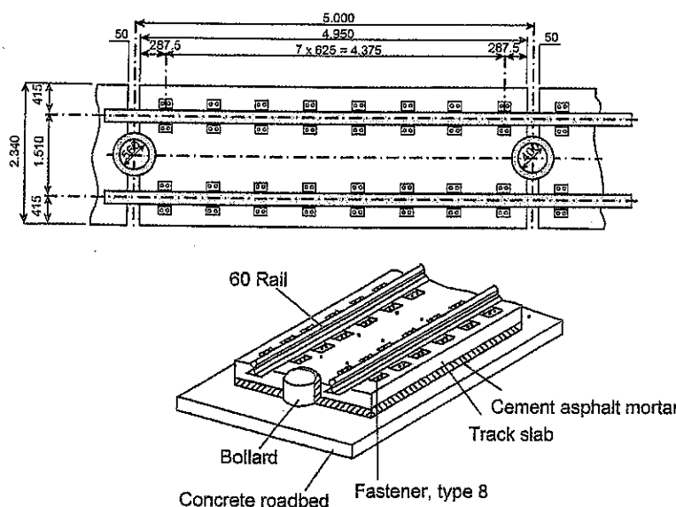
Fig. 1: Shinkansen slab track
