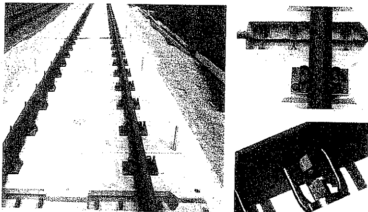
Fig. 3: Bögl slab track system
