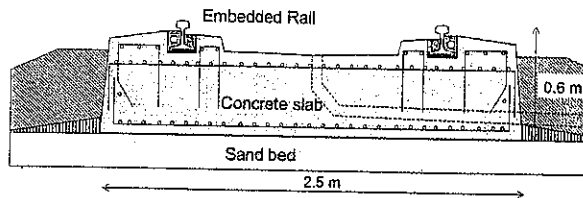
Fig. 5: Embedded rail track near Best (NL)
