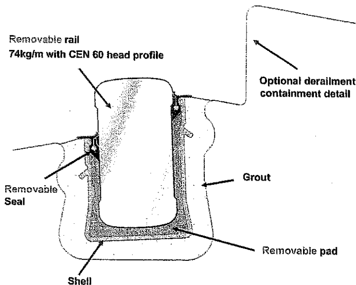
Fig. 7: Balfour Beatty embedded rail
