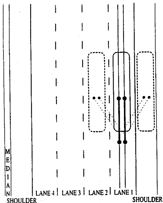
Travel Lane Options - Wires Over Right Lane
